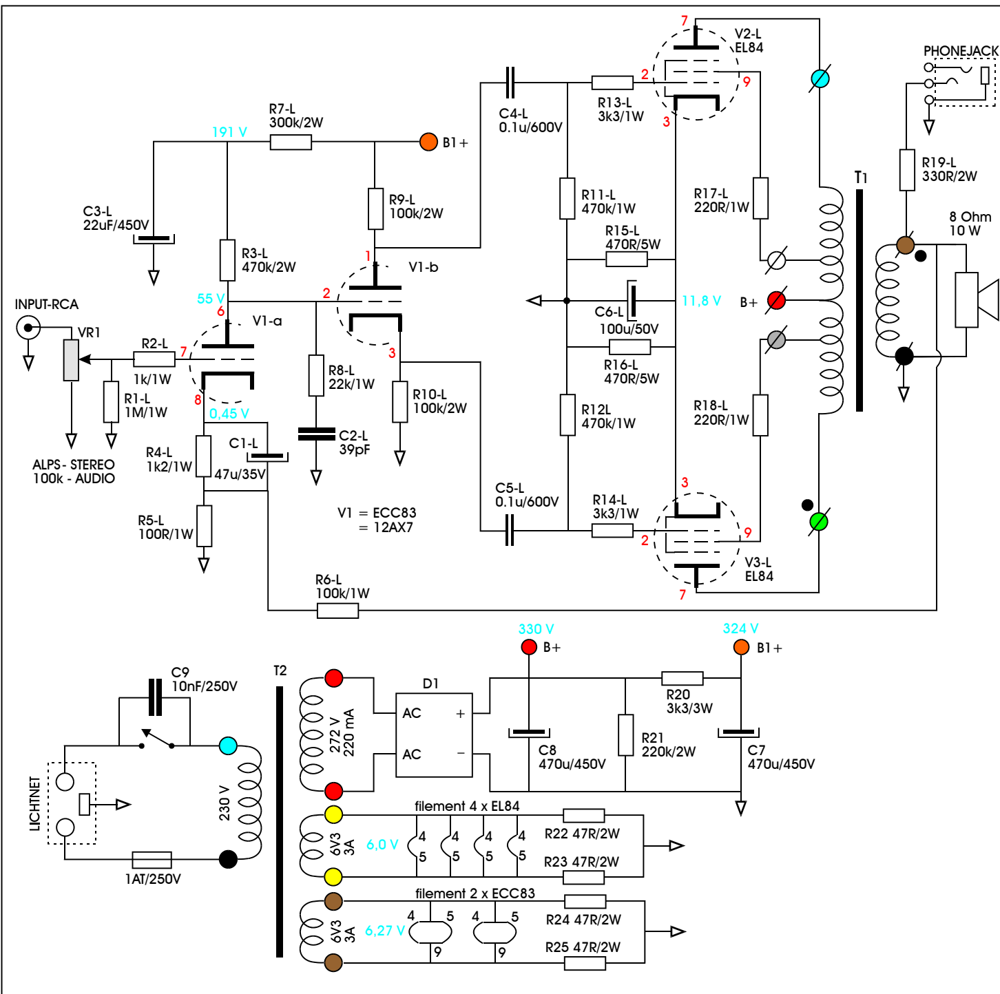
MOD-0 : basis-schema; meting zonder R6,8 C2.
