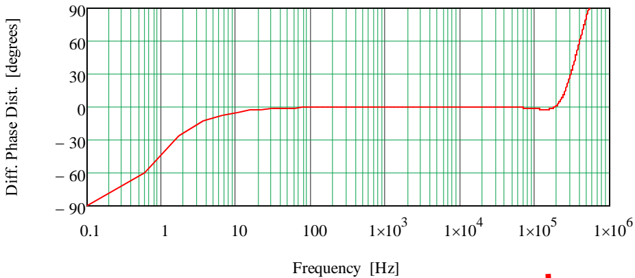
Differential Phase Distortion; vert. 30 deg./div; hor. .1 Hz to 1 MHz
