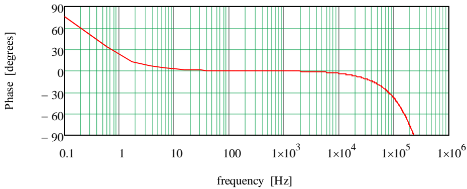
Differential Phase Distortion; vert. 30 deg./div; hor. 0.1 Hz to 1 MHz
