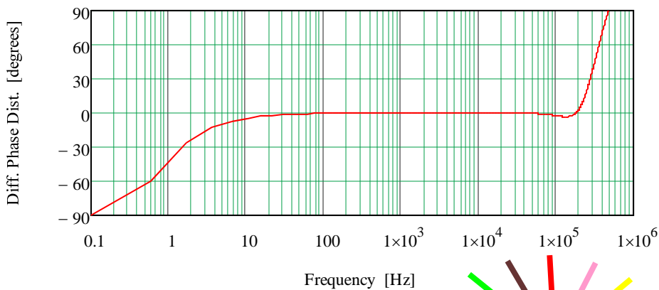
Differential Phase Distortion; vert. 30 deg./div; hor. 0.1 Hz to 1 MHz
