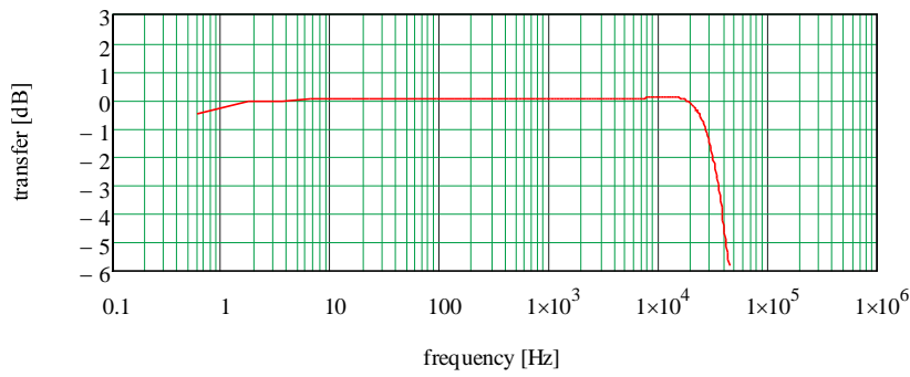
Frequency Response; Vertical 1 dB/div; Horizontal .1 Hz to 1 MHz (3)
