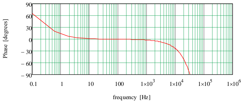
Phase Response; Vertical 30 deg./div; Horizontal .1 Hz to 1 MHz
